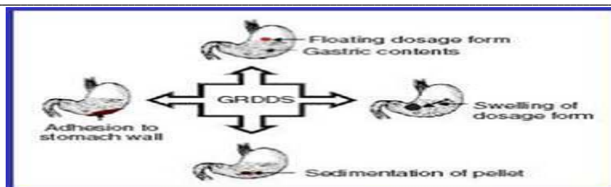
Figure 4: Shows Cycle for Gastroretentive dosage forms
